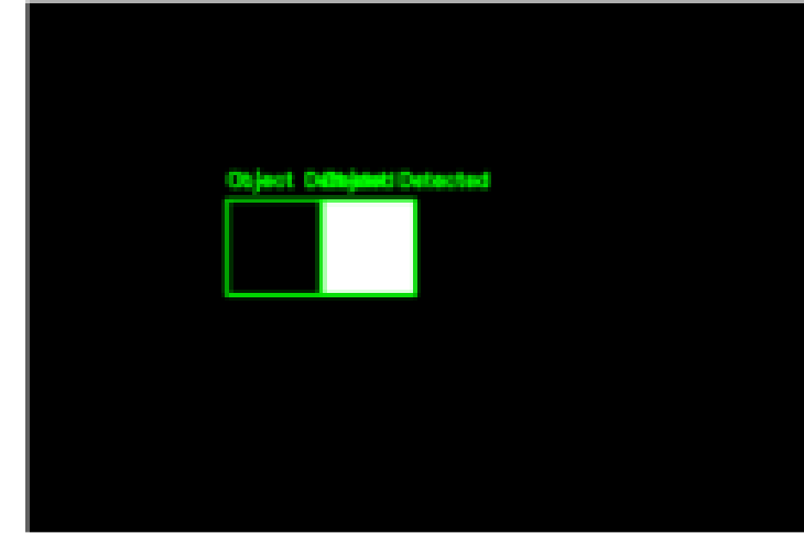
Surveillance Output
