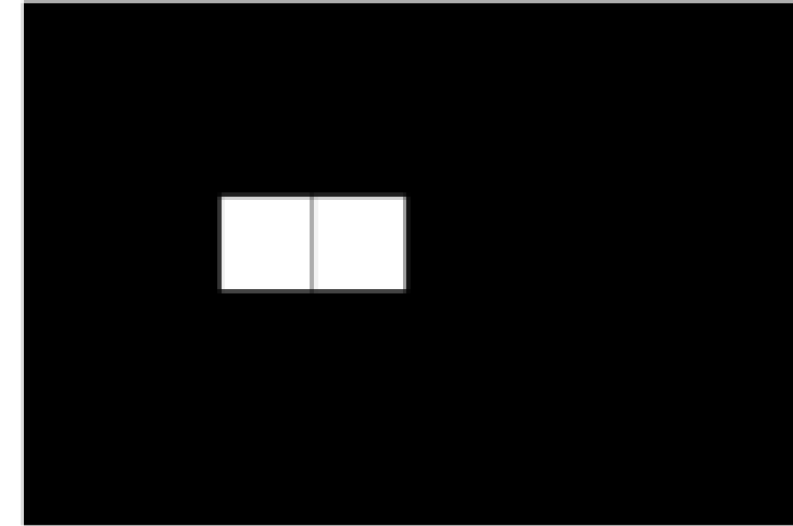
Motion Detection
